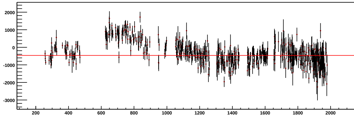
DIA LightCurve in R_Eros band - sm002_7d-62
