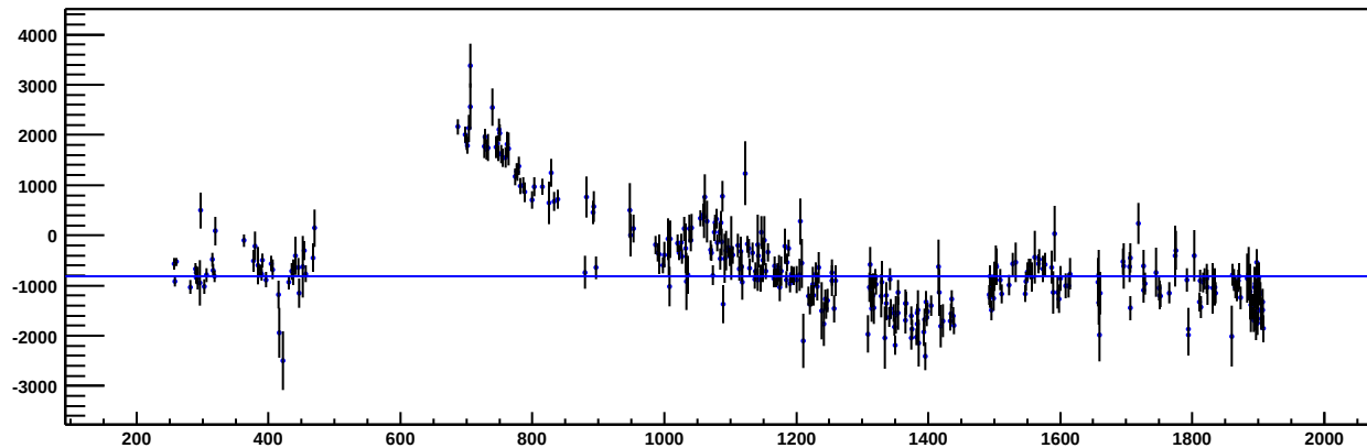
DIA LightCurve in B_Eros band - sm002_7d-62
