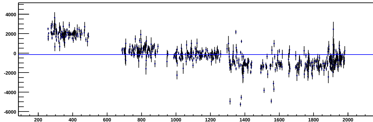
DIA LightCurve in B_Eros band - sm001_6a-74
