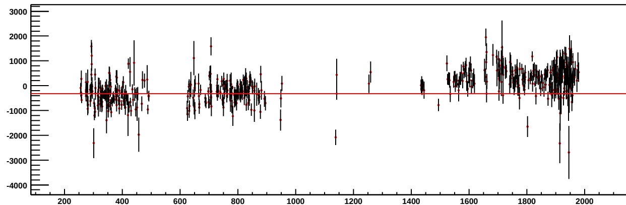
DIA LightCurve in R_Eros band - sm001_66-94
