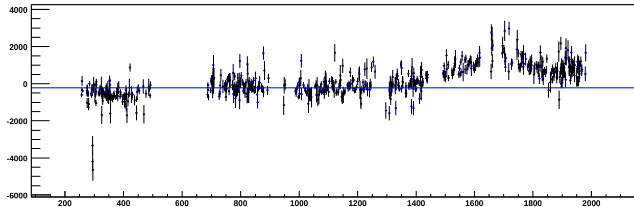
DIA LightCurve in B_Eros band - sm001_66-94
